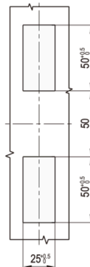
Panel Cutout
